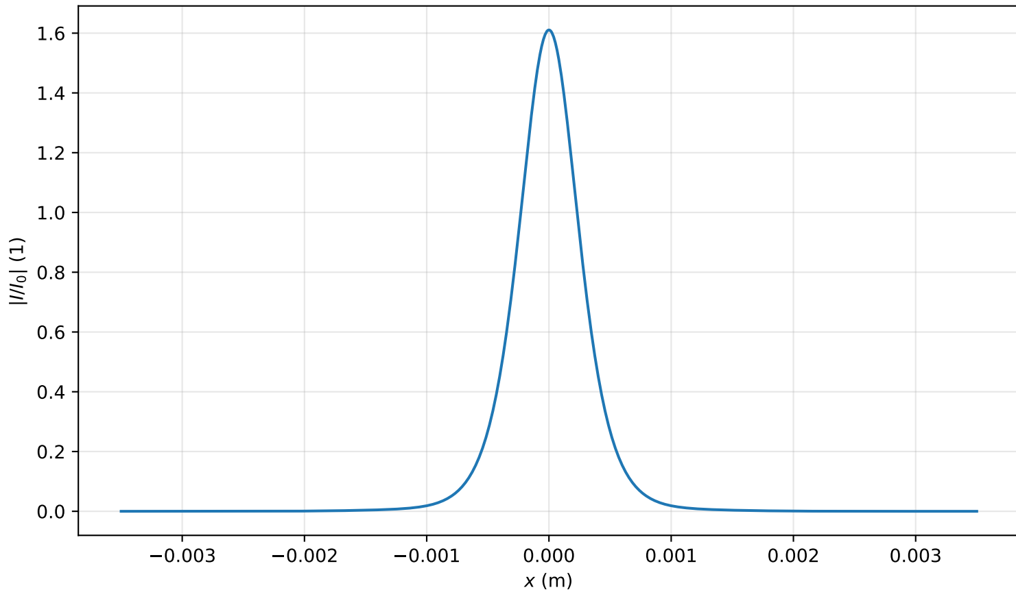
Intensity profile I(x, y = 0, z = 2.627m)/I_0 , P_{in}=0.9P_{cr} , artificial time
